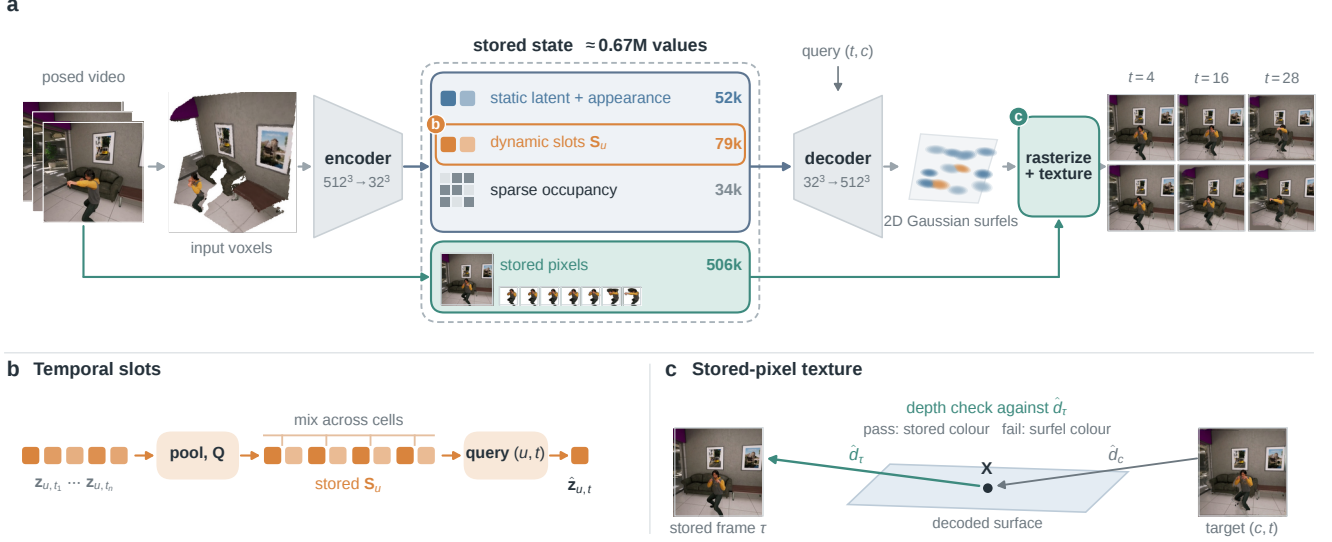
Figure 1. Overview of Sparc4D. (a) Static observations are pooled over the clip and dynamic observations are kept per frame. A shared sparse encoder maps both to a learned state (blue box): static latents and appearance codes, dynamic temporal slots, and the sparse occupancy that guides decoder upsampling. Together with stored source pixels (green box), it forms the stored state (dashed box; mean values per clip, Table 9). At a query time t and camera c , the decoder produces 2D Gaussian surfels that are rasterized and textured. Images are MultiCamVideo inputs and complete-model outputs; the voxels are the clip’s input observations. The marked parts are detailed in (b) and (c). (b) Learned queries \mathbf{Q} pool the per-frame features \mathbf{z}_{u,t} of cell u ; the slots are mixed across cells and stored as \mathbf{S}_u , and a query (u, t) decodes \hat{\mathbf{z}}_{u,t} . Latent and appearance features use separate slots with 32 and 4 channels. (c) A target pixel is back-projected with the rendered depth \hat{d}_c to \mathbf{X} and takes the colour of a stored frame \tau if the depth \hat{d}_\tau rendered there agrees; otherwise it keeps the surfel colour. Geometry is unchanged.
