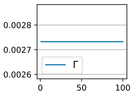
Batch Size
