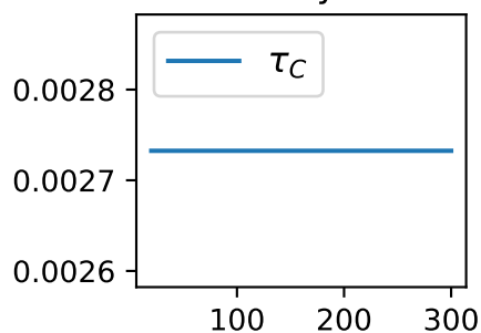
Concurrency Number
