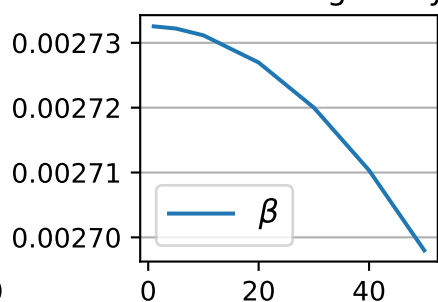
Gradient Smooth
