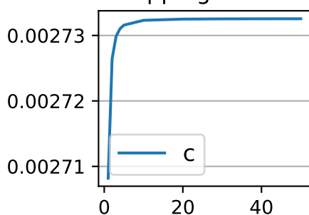
Aggregate Number
