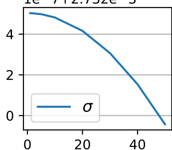
Concurrency Number
