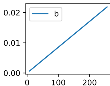
Batch Size
