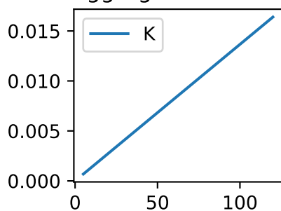
Aggregate Number
