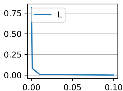
Gradient Smooth
