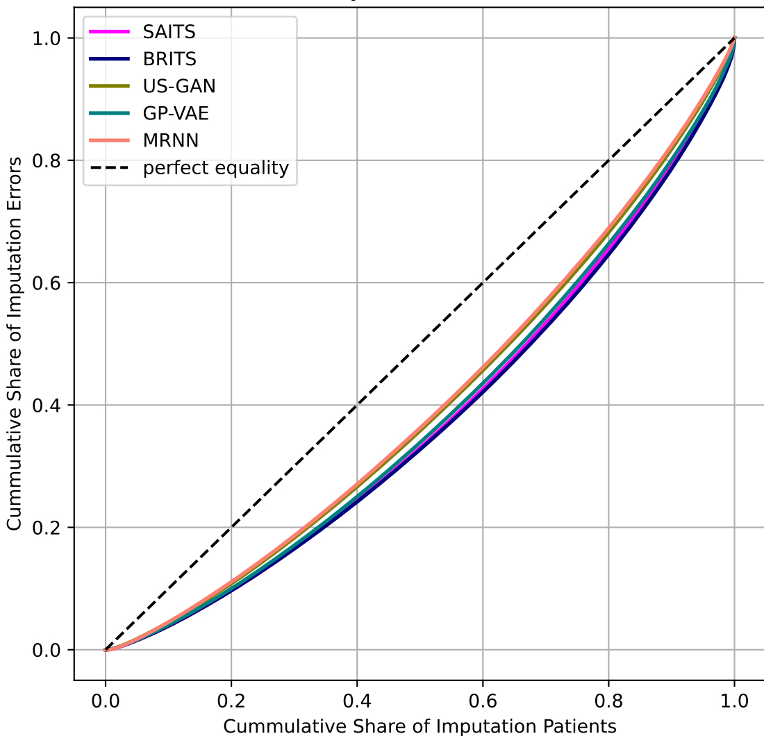
Lorenz Curves by Model for All Models - Male
