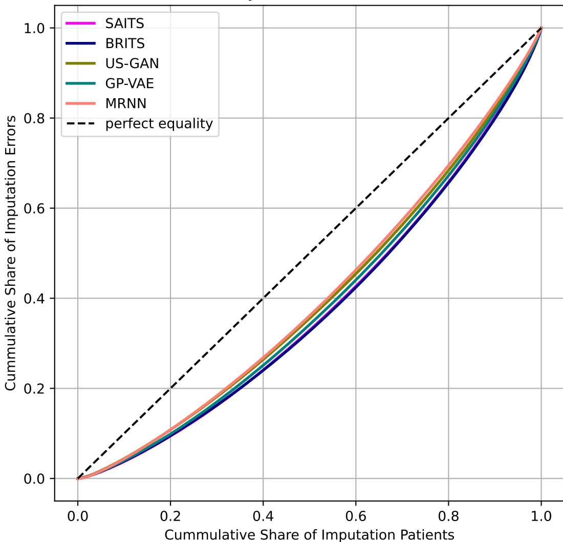
Lorenz Curves by Model for All Models - Female
