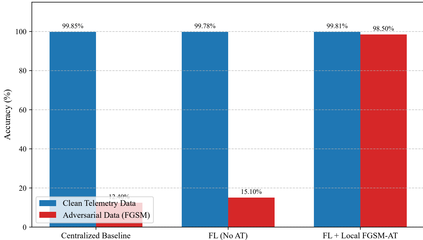
Accuracy Under Evasion Attack (FGSM, \epsilon=0.1 )
