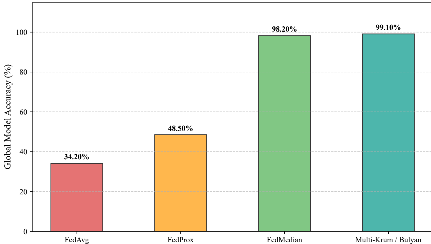
Global Accuracy Under Model Poisoning Attack (1 Malicious Client)
