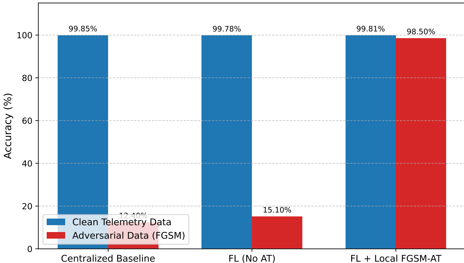
Accuracy Under Evasion Attack (FGSM, eps=0.1)
