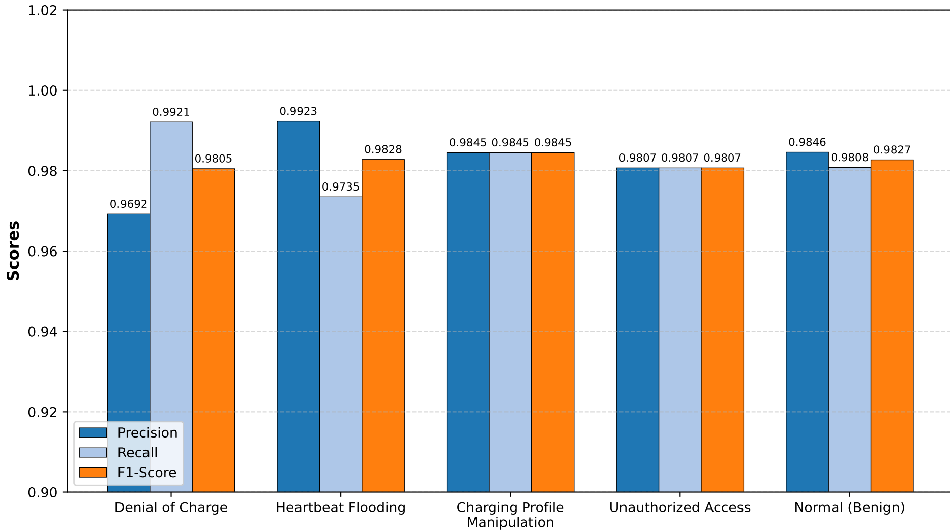
Baseline FIDS Classifier Performance Metrics (Scenario A)
