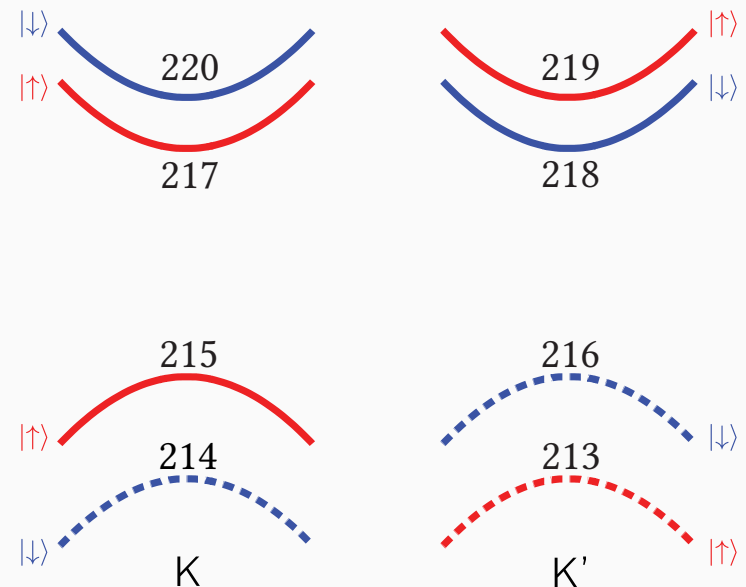
MoSe 2 band index.
