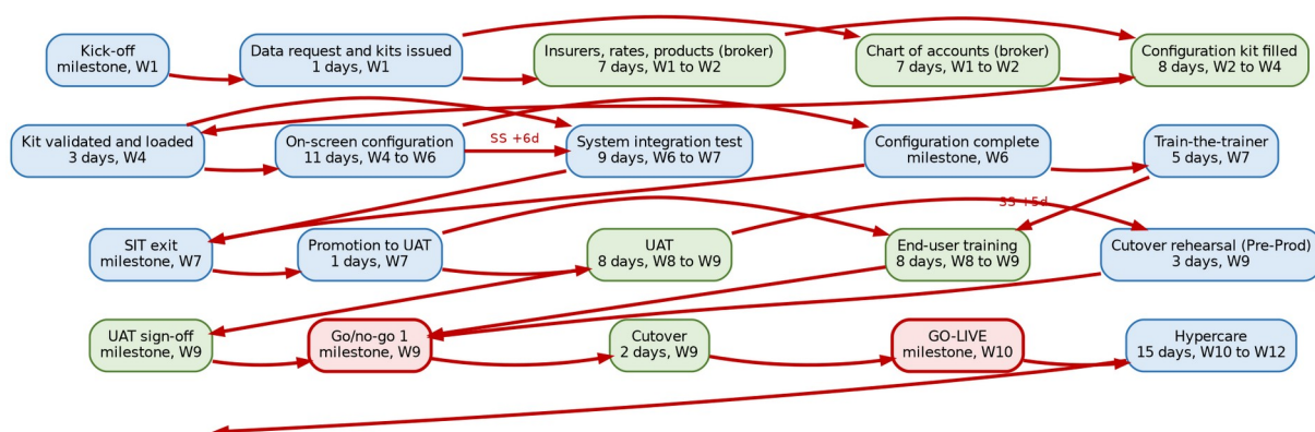
Critical path of a medium broker
