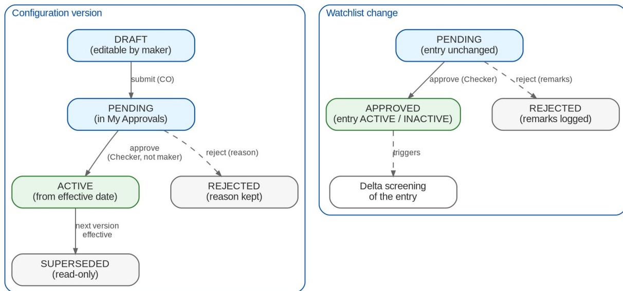
Figure 3: Maker-checker states of configuration versions and list changes (SNSRP-101 to 109, 203, 204)
