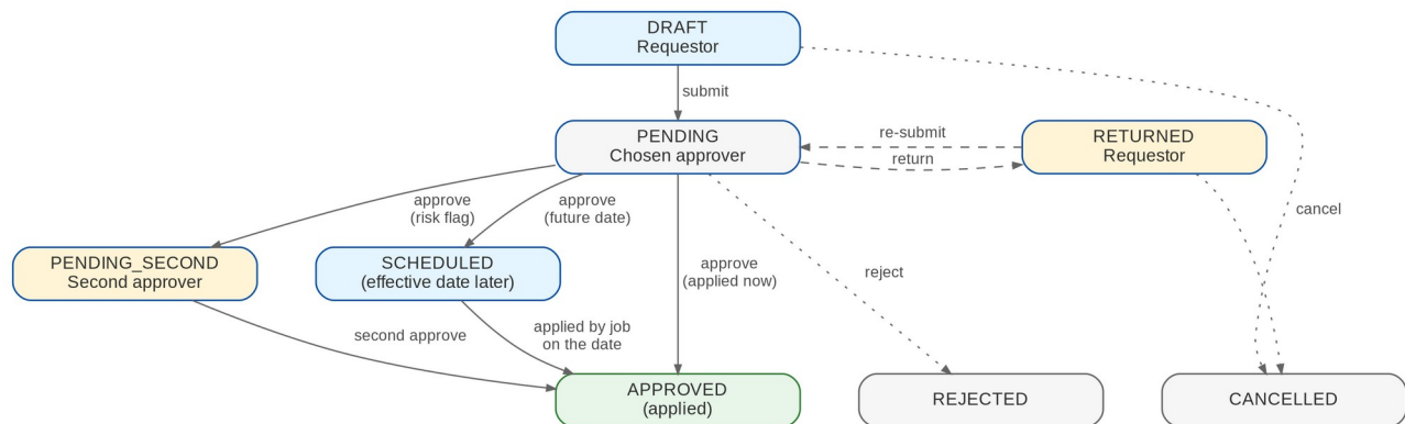
Figure 2: Status of a user access request (BRD 1.002-1.009, 2.002)
