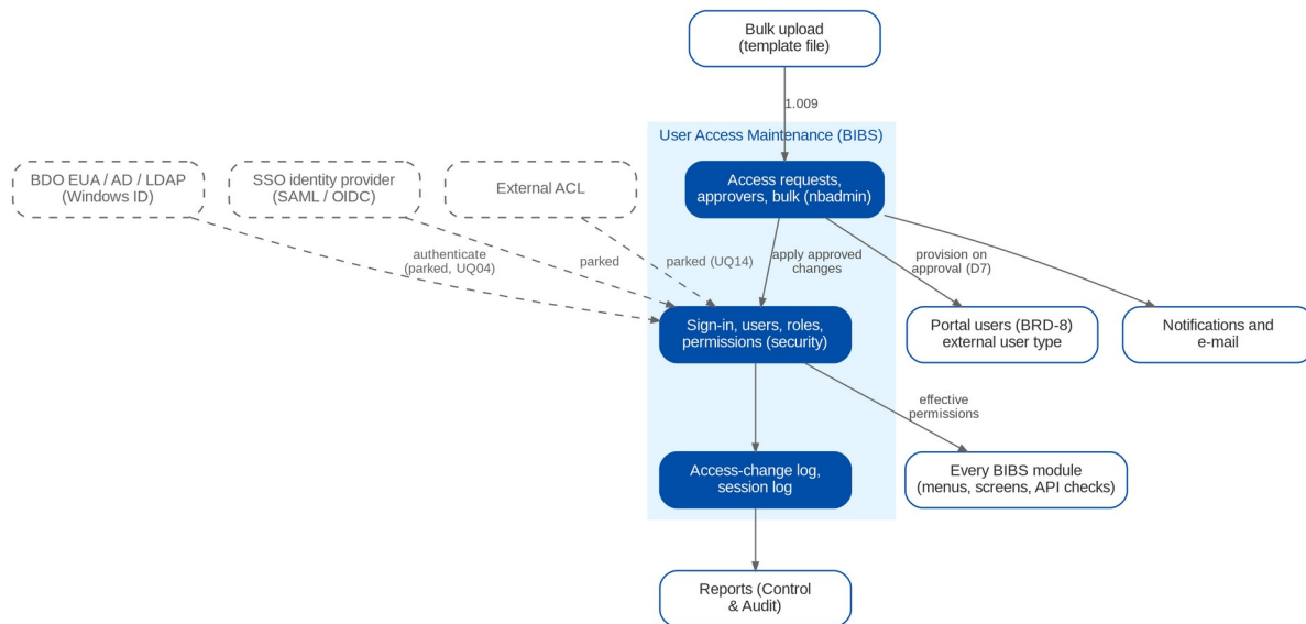
Figure 4: Interfaces of User Access Maintenance (dashed = parked)
