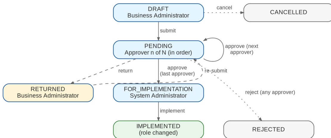
Figure 3: Status of a group-profile request (BRD 3.002; p.6)
