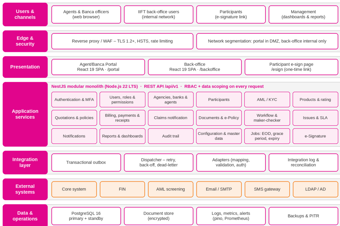
Figure 111: SalesVerse 2.0 logical architecture
