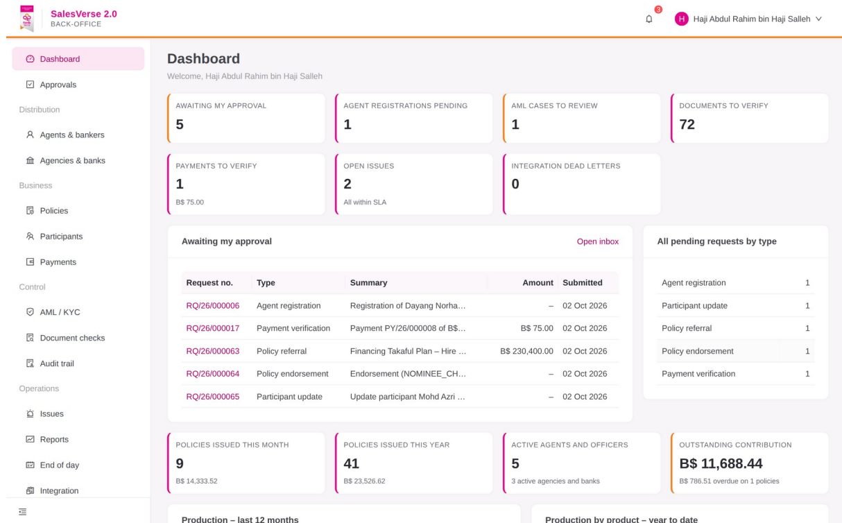
Figure 1: Management dashboard: Month and year-to-date issuance, outstanding contribution, production trend, split by product and channel.
