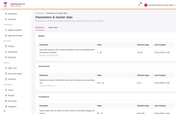
Figure 94: Parameters: Parameters by category with allowed range and last change.
