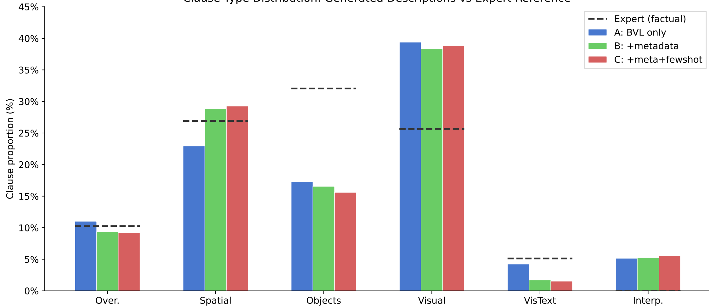
Clause Type Distribution: Generated Descriptions vs Expert Reference
