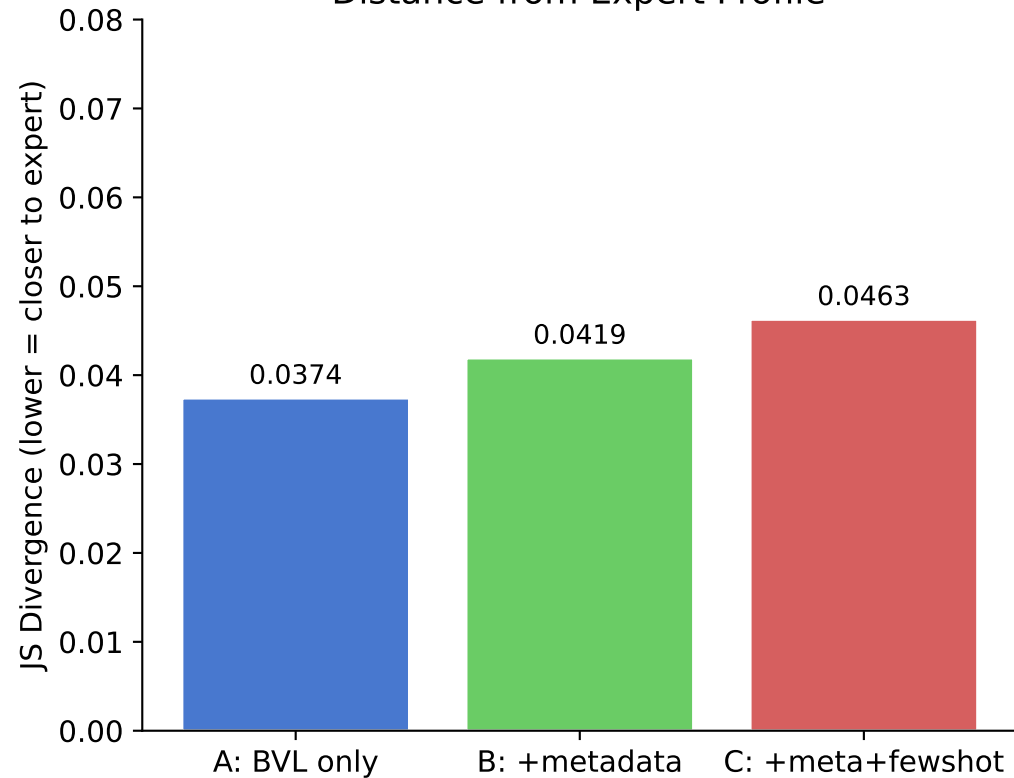
Distance from Expert Profile
