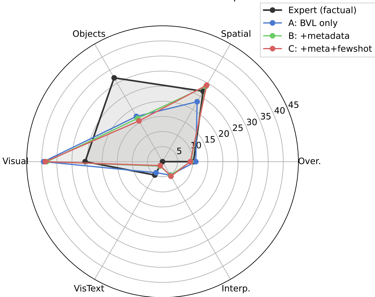
Clause Profile: Generated vs Expert
