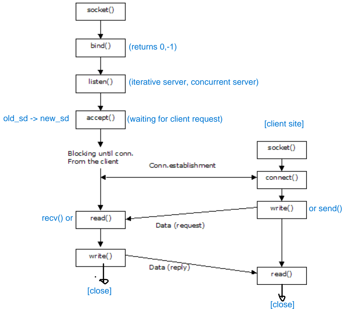
Fig. 3. Socket system calls for connection-oriented case.
