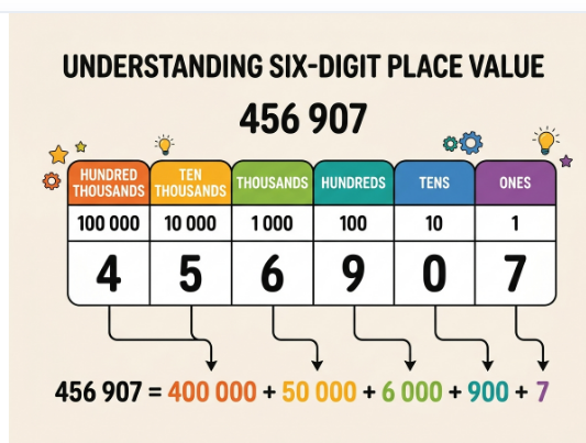
Six-digit place-value chart
