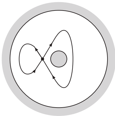
Figure 4.10.4: Two loops in an annular region that cannot be homotopic.
