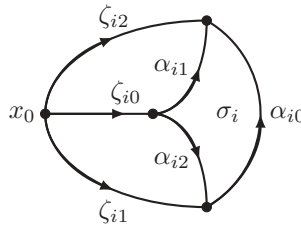
Figure 4.10.8: The simplex \sigma_i , its edges \alpha_{i0}, \alpha_{i1}, \alpha_{i2} , and the paths \zeta_{i0}, \zeta_{i1}, \zeta_{i2} connecting the base point x_0 to the vertices of \sigma_i .
