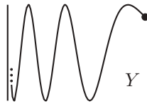
The Topologist's Sine Curve
