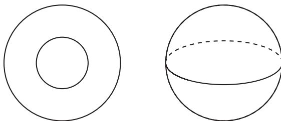
Figure 4.10.1: Different types of holes.
