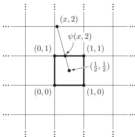
Figure 4.10.12: The map \psi .
