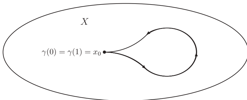
Figure 4.10.2: A loop in X .
