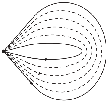
Figure 4.10.3: A pair of homotopic loops.
