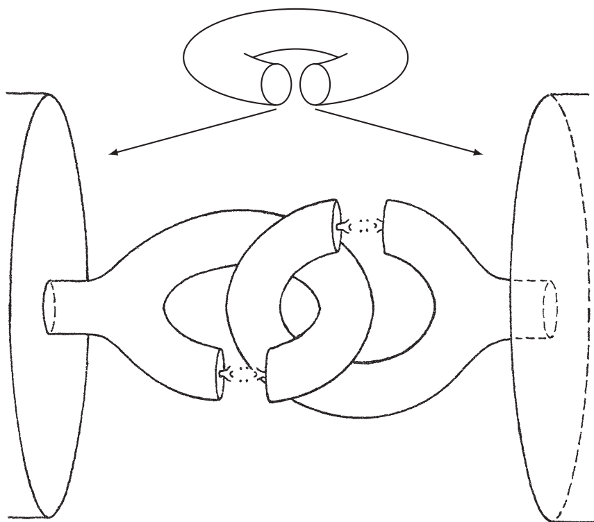
Alexander Horned Sphere Figure 4.9.4
