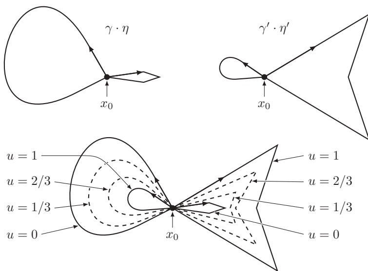
Figure 4.10.6: Homotopy from \gamma \cdot \eta to \gamma' \cdot \eta' .
