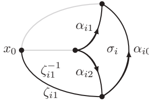
Figure 4.10.10: The loop \beta_i .
