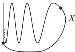
The Closed Topologist's Sine Curve Figure 4.6.1
