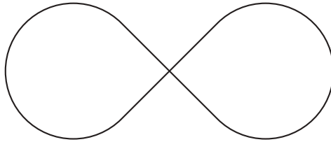
Figure 4.10.11: The figure 8 space.
