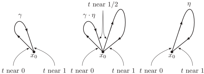
Figure 4.10.5: The product of \gamma and \eta .
