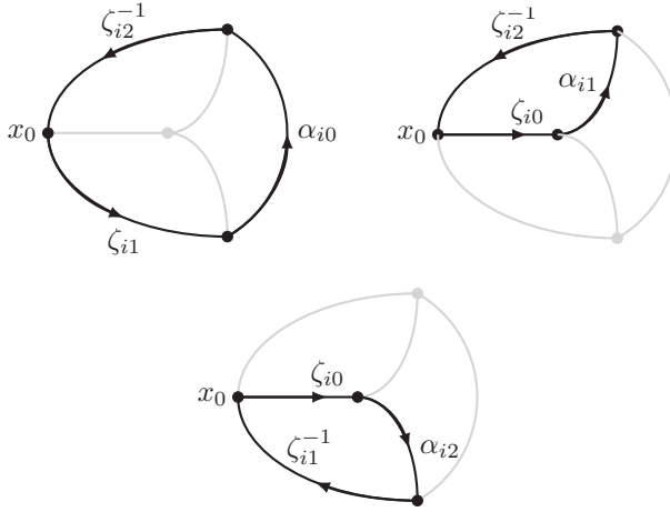
Figure 4.10.9: The loops \beta_{i0}, \beta_{i1}, \beta_{i2} .
