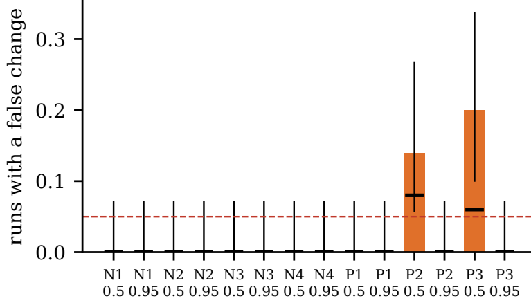
Figure 5: Fraction of runs with at least one false change (Clopper–Pearson 95% CI) per scenario and input persistence; dash: fraction where it remained at the end. Blue: nulls; orange: one true input.
