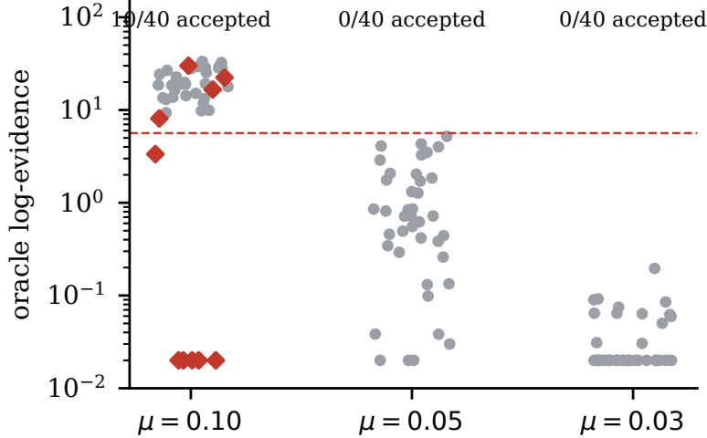
Figure 2: Structureless targets with real inputs (development, 120 runs). Log-evidence of the best fixed-coefficient challenger (projection oracle) versus the threshold (dashed); red: runs where the model actually accepted a change. The median oracle crosses the threshold at \mu = 0.1 (18.2) and stays below it at \mu = 0.05 (maximum 5.2).
