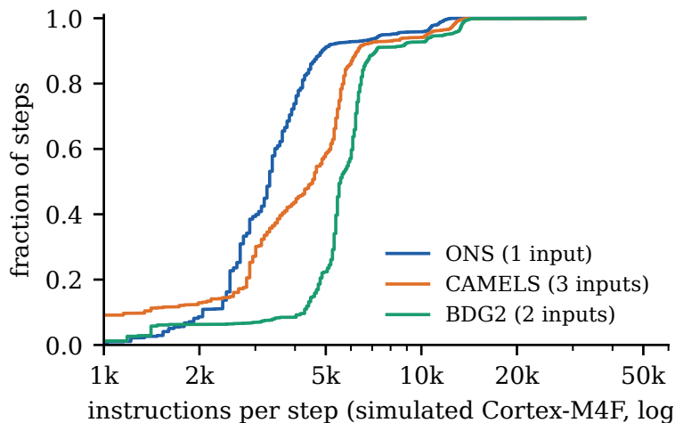
Figure 4: Cumulative distribution of instructions per step on three development series (simulated Cortex-M4F). The cheapest steps have a missing target.
