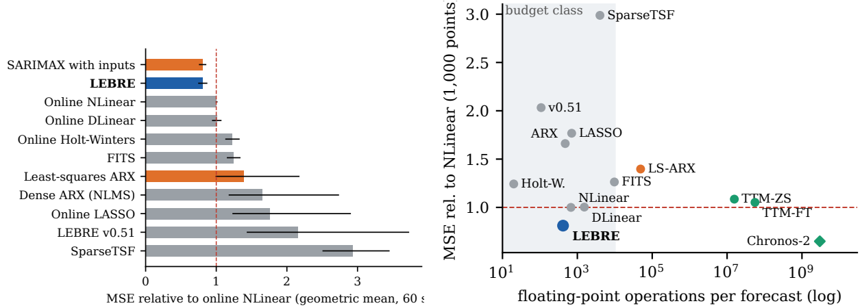
Figure 3: Reserve 3 (60 never-seen series). Left: MSE relative to online NLinear with 95% CIs (blue: LEBRE; grey: budget class; orange: classical references). Right: error on the 1,000-point protocol versus operations per forecast; the grey band is the budget class. SARIMAX is omitted on the right because its per-forecast cost was not counted. The Chronos-2 cost (diamond) is an order-of-magnitude estimate.
