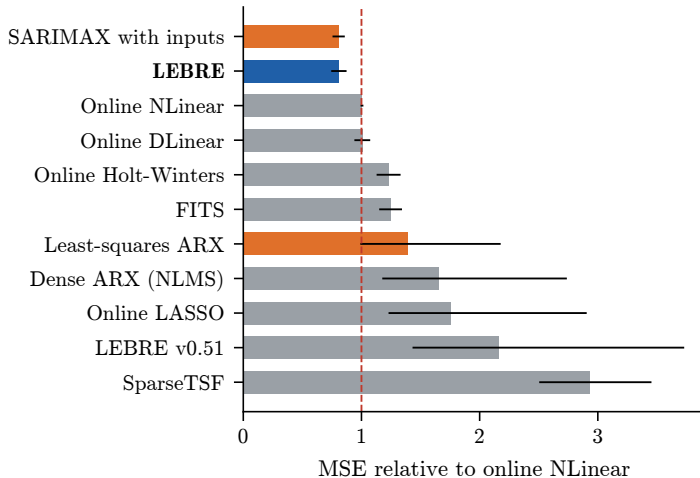
(a) accuracy, 60 series (95% CI)
