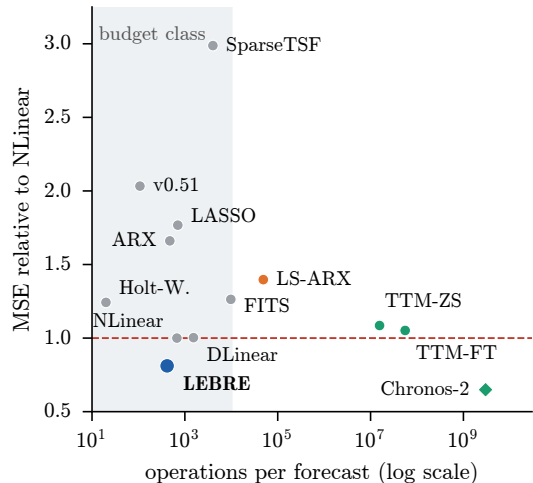
(b) accuracy vs. cost, 1,000-point protocol
