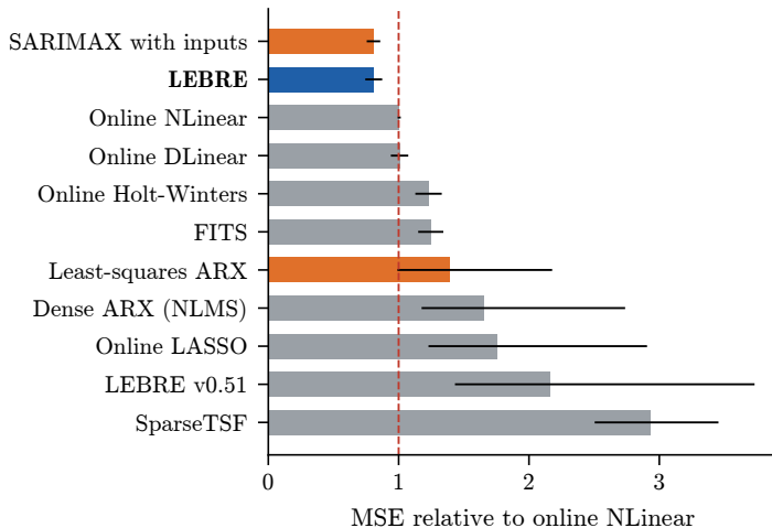
(a) accuracy, 60 series (95% CI)
