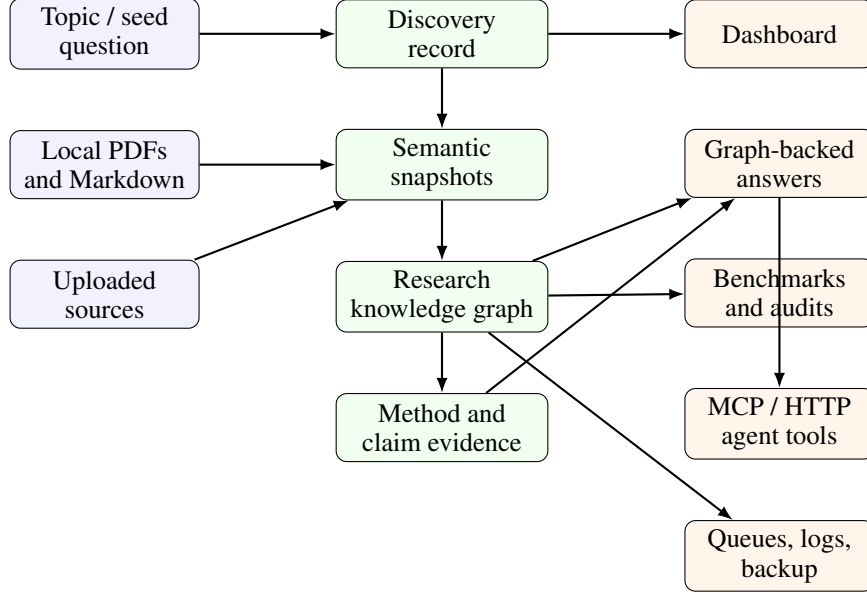
Figure 1: Functional view of PAPERNEXUS. Discovery, ingestion, graph memory, evidence, benchmark, agent, and operations layers are maintained as local artifacts or controlled interfaces without changing the local ownership model.
