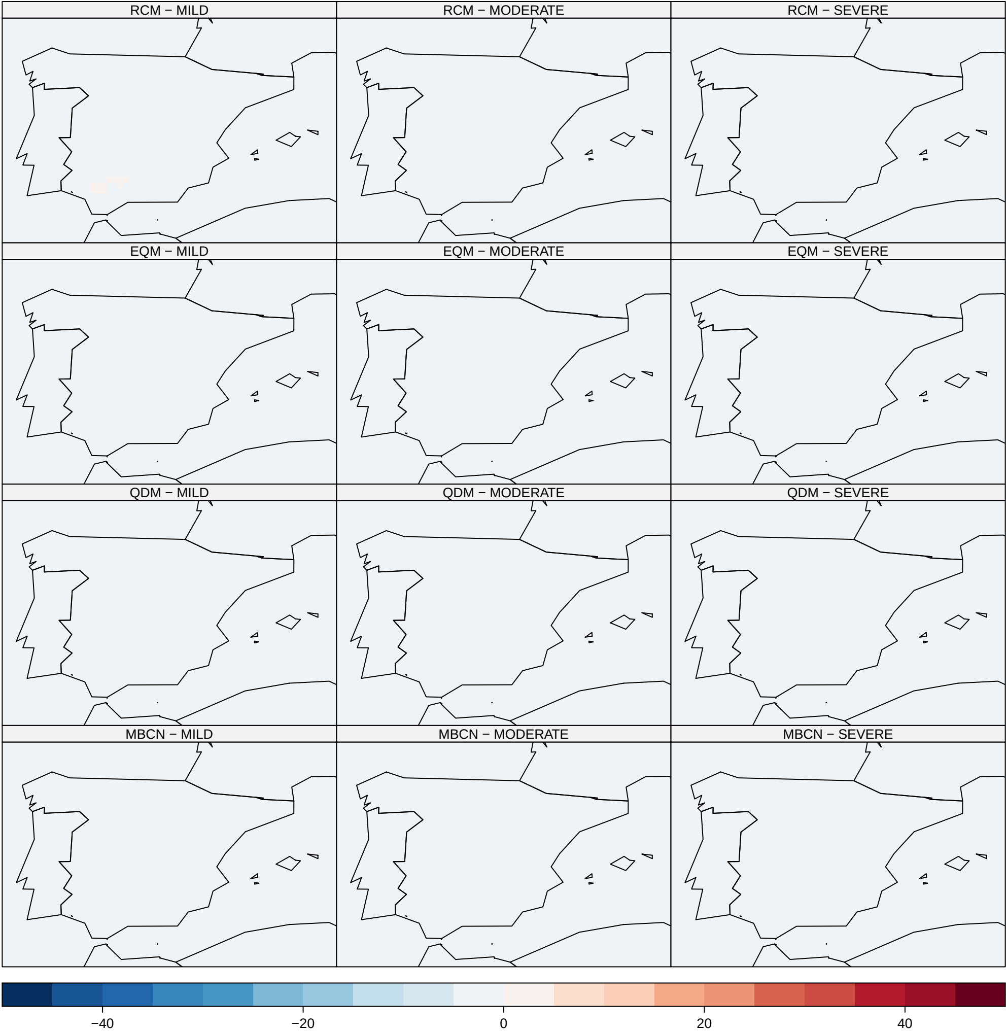
Delta no. of days within stress class
