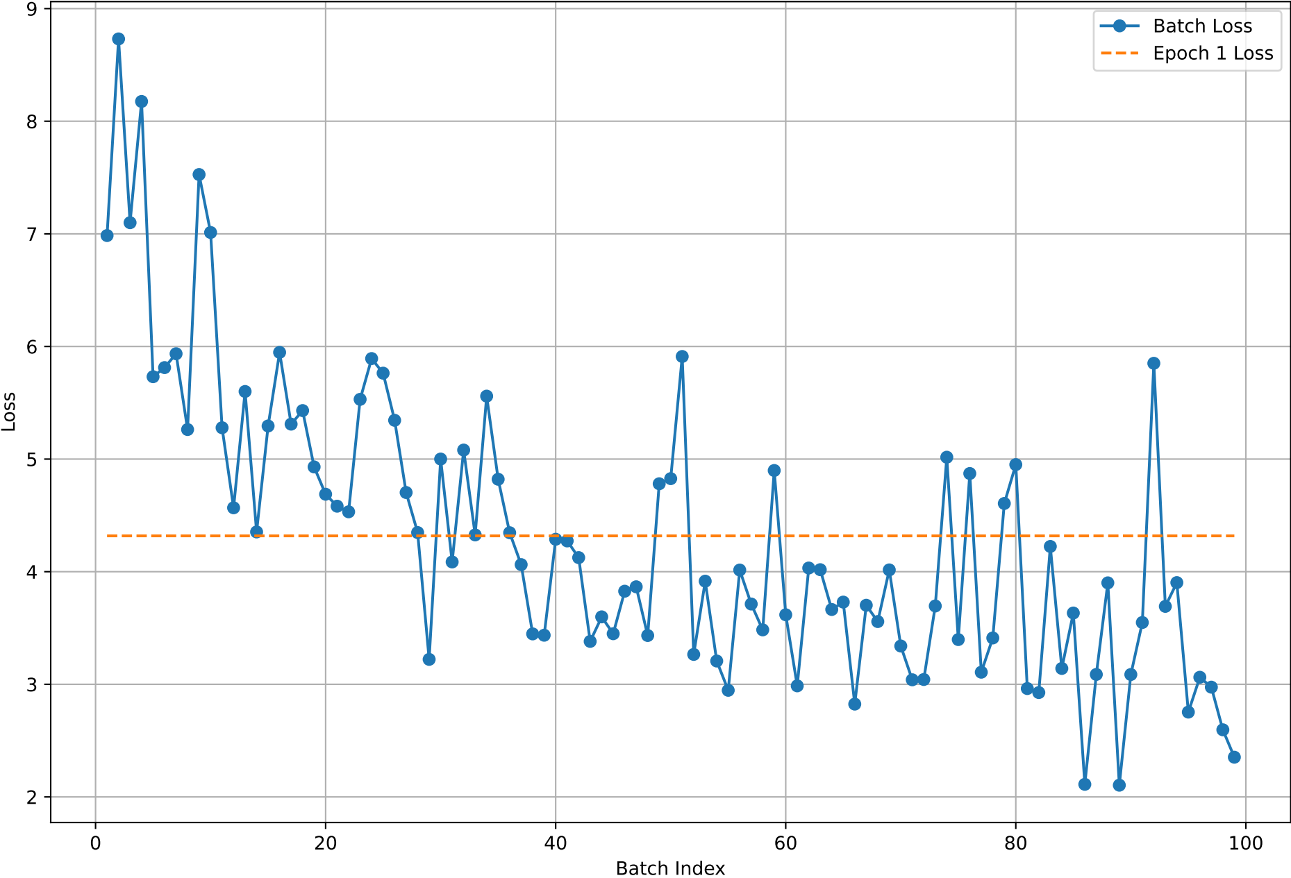
Batch vs. Epoch Loss (Epoch 1)
