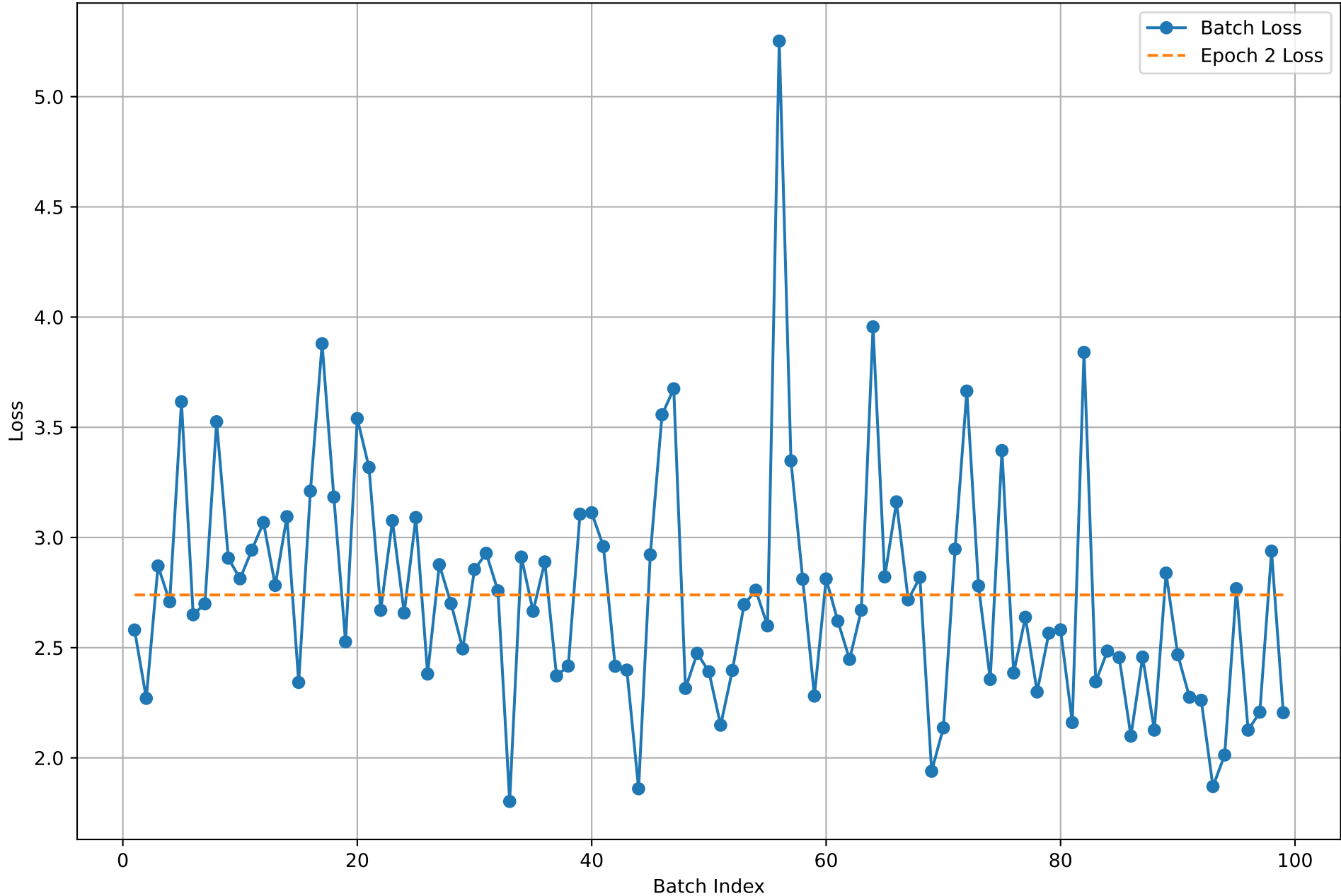
Batch vs. Epoch Loss (Epoch 2)
