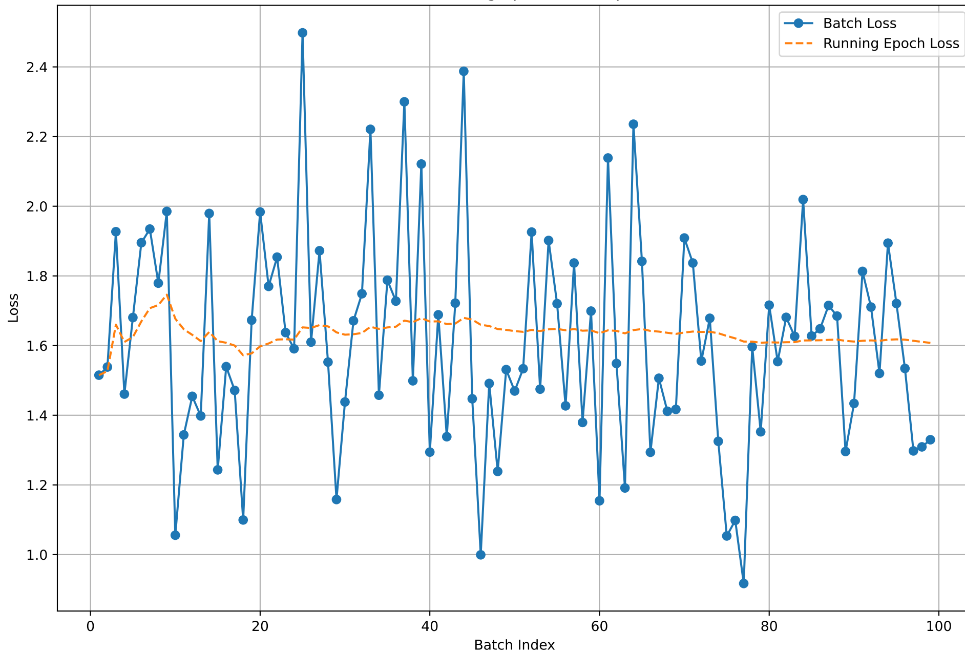
Batch and Running Epoch Loss (Epoch 10)
