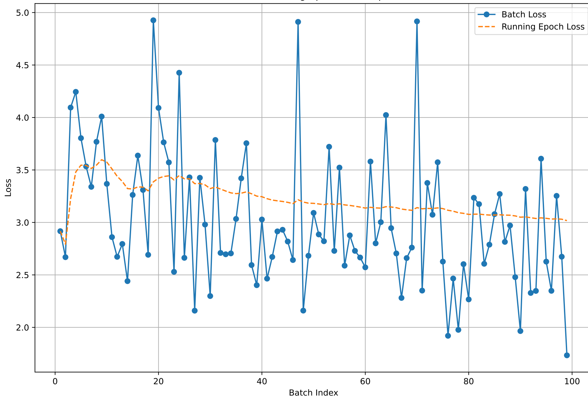
Batch and Running Epoch Loss (Epoch 2)
