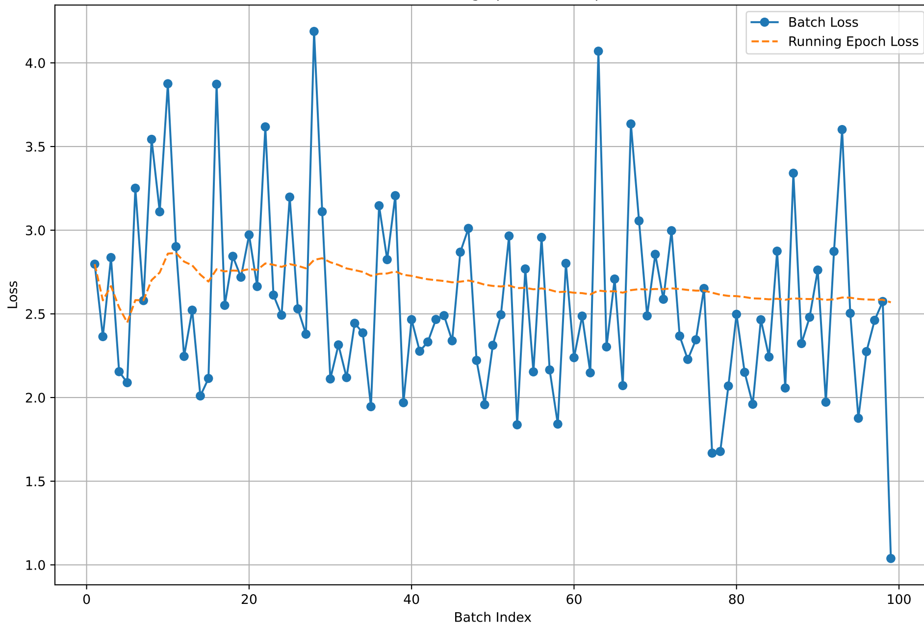
Batch and Running Epoch Loss (Epoch 3)
