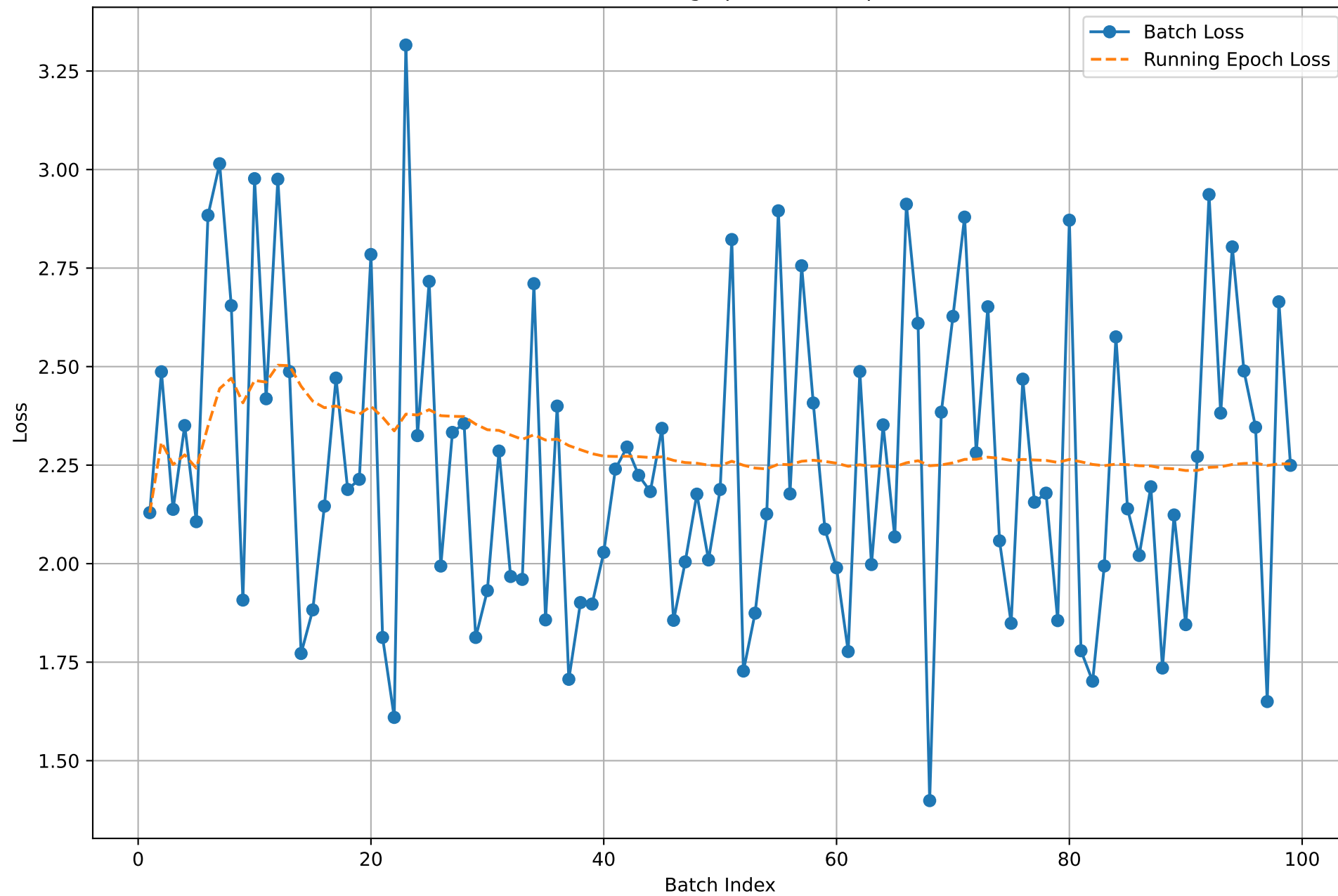
Batch and Running Epoch Loss (Epoch 4)
