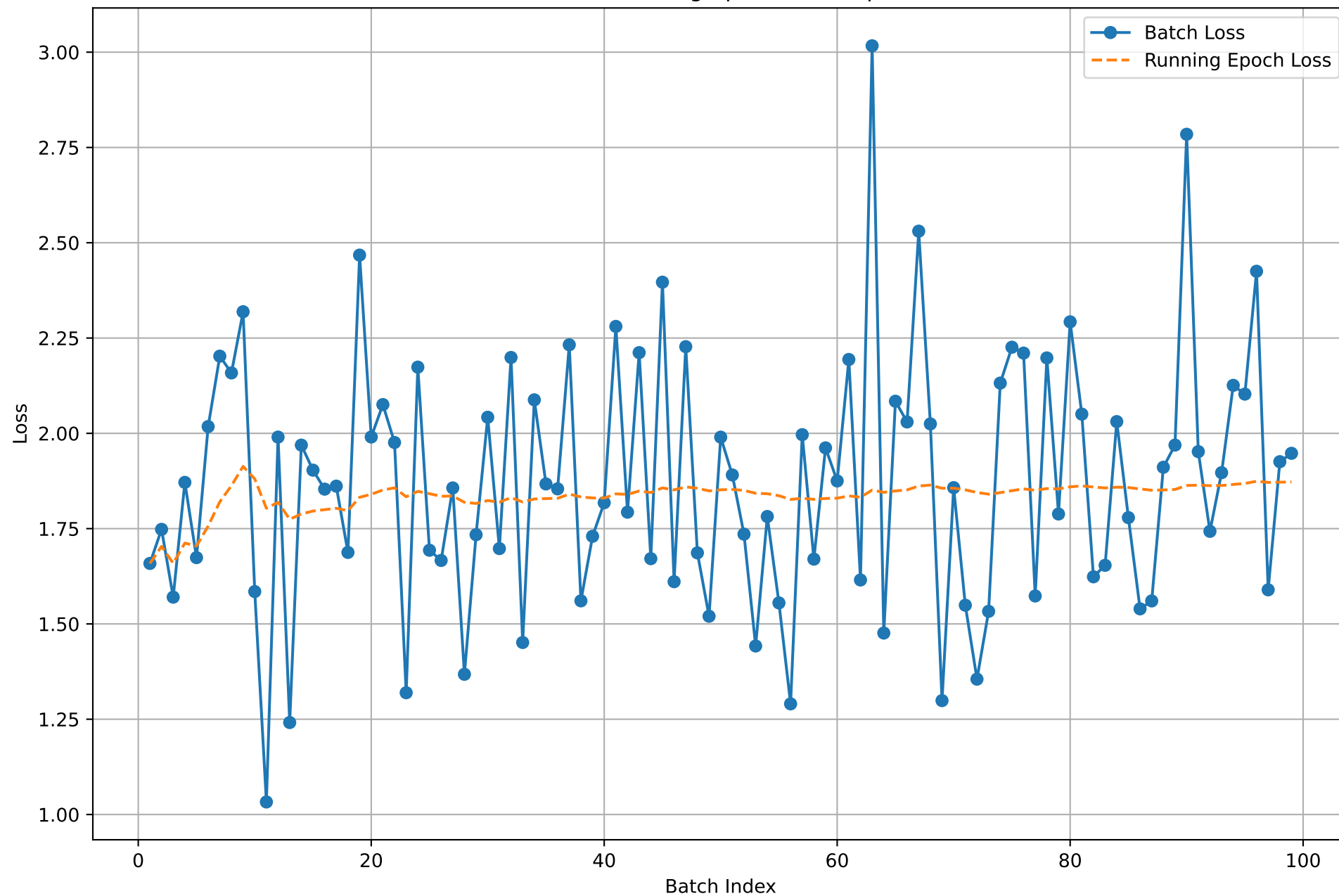
Batch and Running Epoch Loss (Epoch 6)
