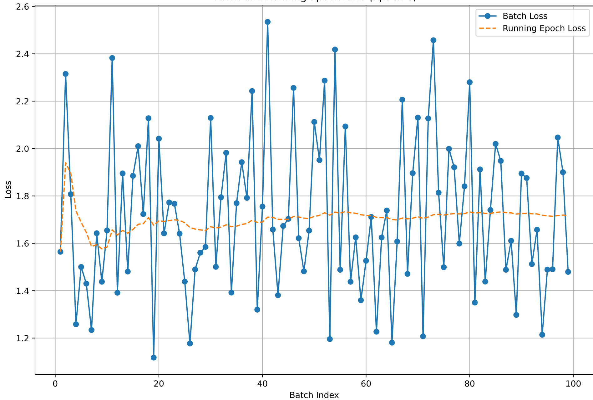
Batch and Running Epoch Loss (Epoch 8)
