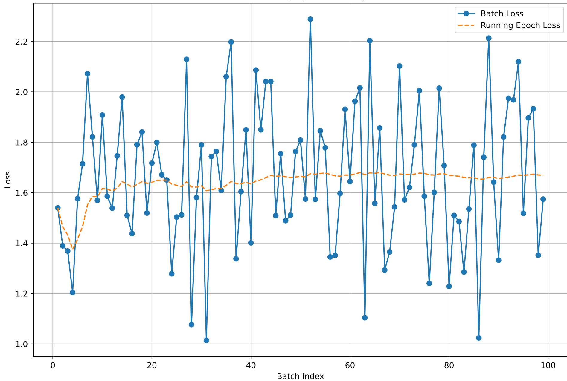
Batch and Running Epoch Loss (Epoch 9)
