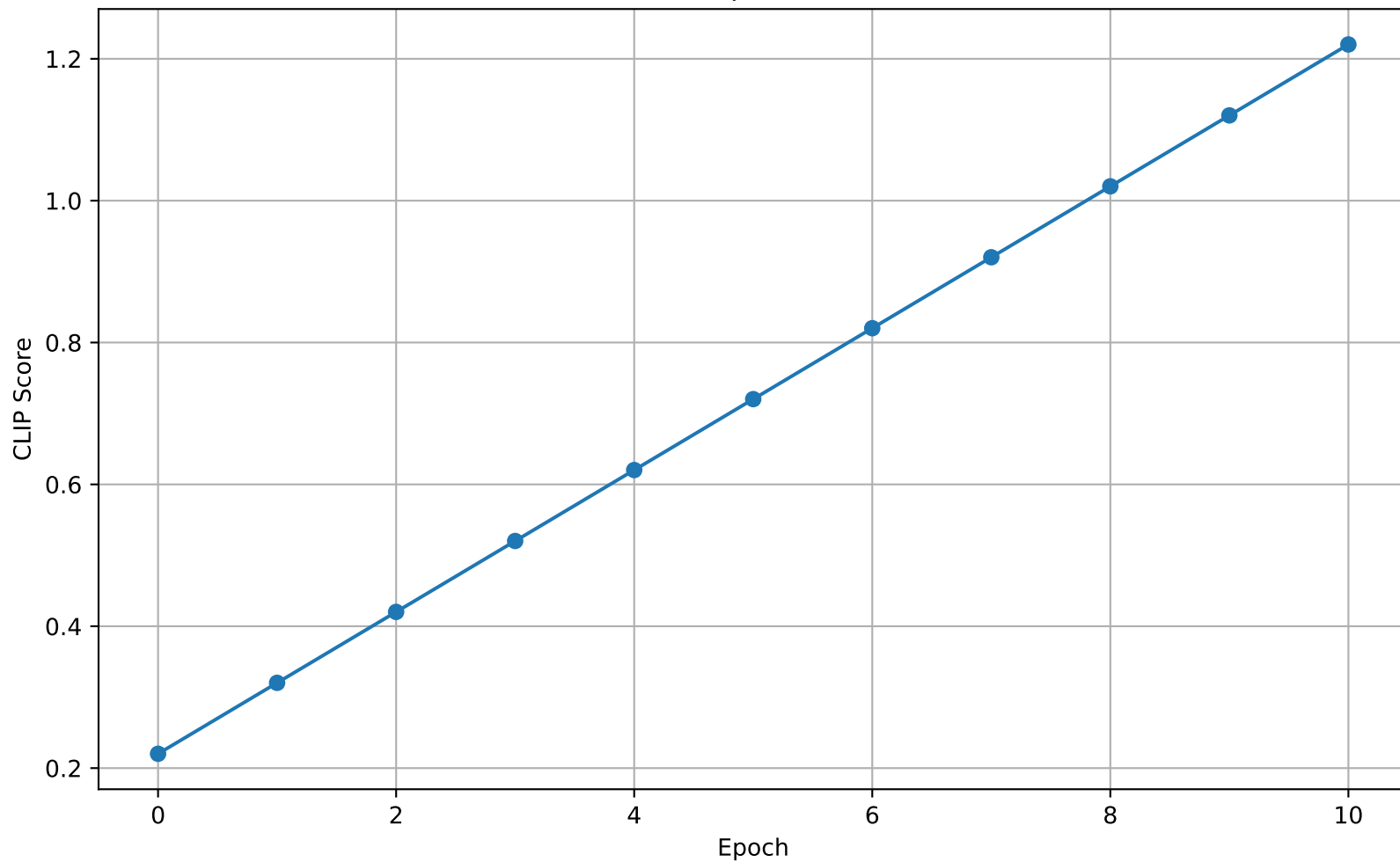
CLIP Score Over Epochs (Baseline at 0)
