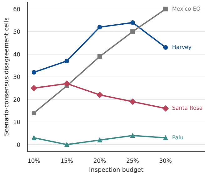
Exact-budget sensitivity
