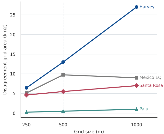
Disagreement area across grid scales
