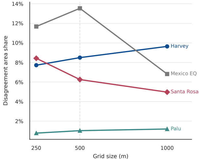
Disagreement area share across grid scales
