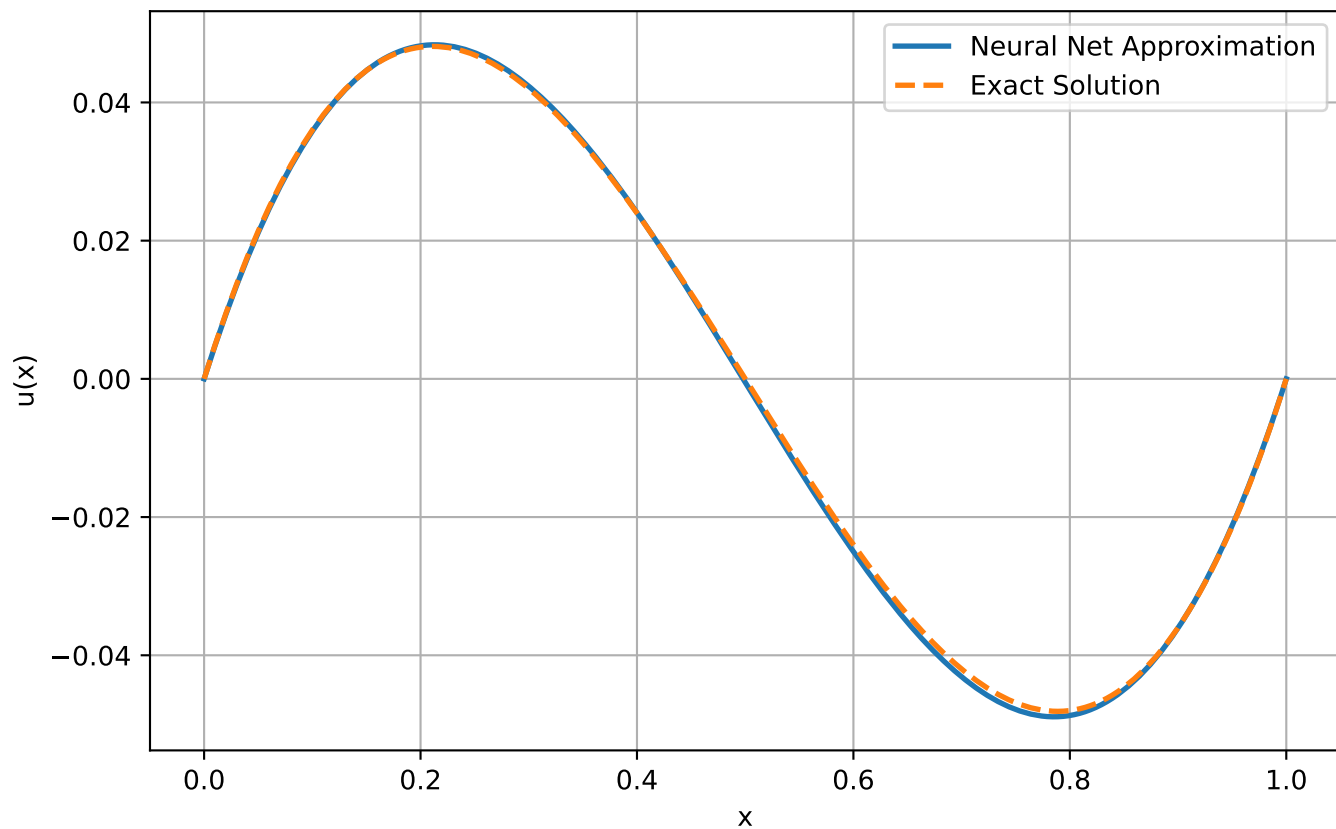
Solution to -u''(x) = -6x + 3 with u(0)=u(1)=0
