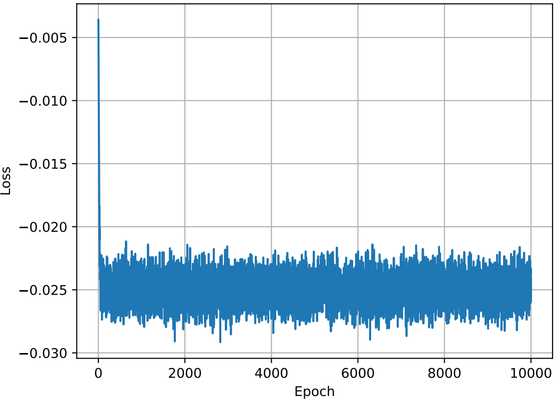
Training Loss
