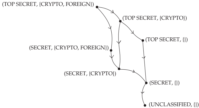
Figure 10.3: A lattice of security labels
