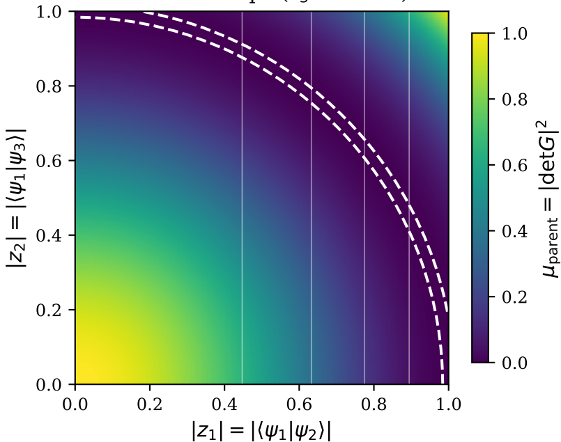
Born landscape ( z_3 = 0 slice)
