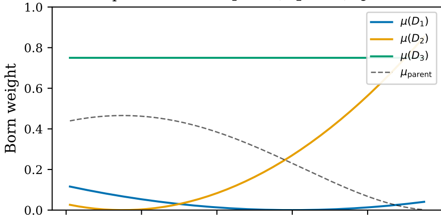
Spectator fiber: z_1 = 0.5 , z_2 = 0.3 , z_3 = t
