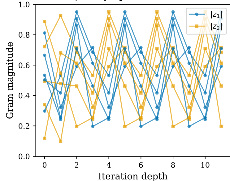
D_3 -always: period 3 (Thm A)
