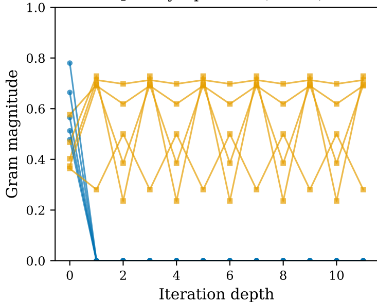
D_1 -always: period 2 (Thm B)
