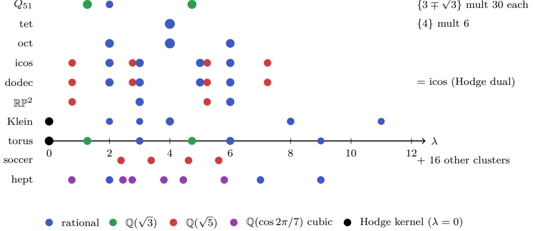
Figure 13: L_1 spectra across the 10-substrate corpus. Each row plots the distinct eigenvalues of L_1(X) on the \lambda -axis as coloured dots; multiplicities are not encoded by dot size (see Table 10 for full multiplicities). Colour encodes Galois content: rational eigenvalues in blue; \mathbb{Q}(\sqrt{3}) Galois pairs in green; \mathbb{Q}(\sqrt{5}) pairs in red; cubic \mathbb{Q}(\cos 2\pi/7) orbits in purple. Black dots at \lambda = 0 mark the Hodge kernel on the Klein bottle (kernel dim 1) and torus (kernel dim 2). The same \mathbb{Q}(\sqrt{3}) pair \{3 \pm \sqrt{3}\} appears in both Q_{51} and the torus T_{3,3}^2 . All four A_5 substrates (icos, dodec, \mathbb{RP}^2 , soccer) carry \mathbb{Q}(\sqrt{5}) pairs with substrate-dependent rational coefficients (icos: \{3 \pm \sqrt{5}, 5 \pm \sqrt{5}\} ; soccer: \{(7 \pm \sqrt{5})/2, (9 \pm \sqrt{5})/2\} ). The heptagonal bipyramid exhibits the only cubic orbits.
