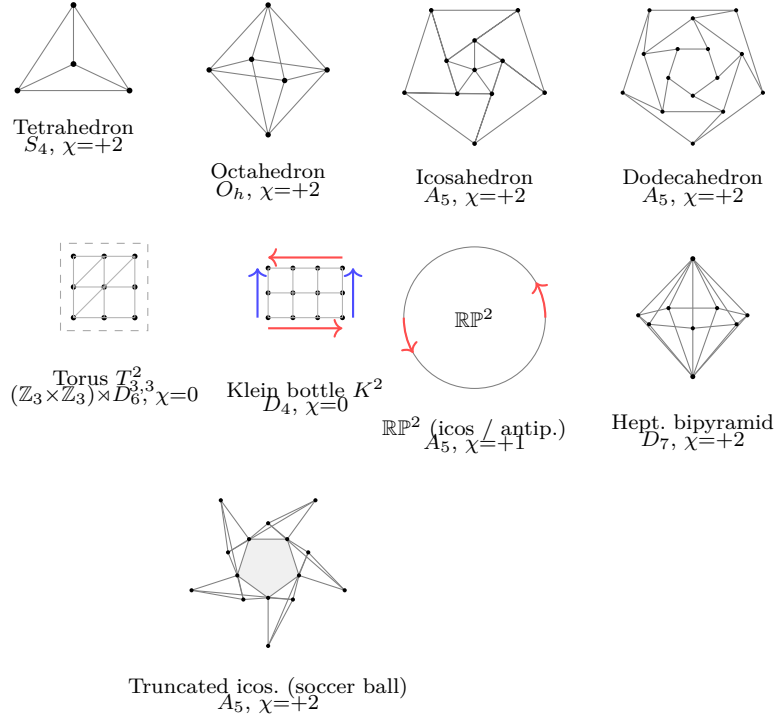
Figure 8: The nine substrates studied in Part 2. Top row: tetrahedron, octahedron, icosahedron, dodecahedron (the Platonic family and its A_5 -symmetric Hodge dual); second row: surface quotients (torus T_{3,3}^2 , Klein bottle K^2 , \mathbb{RP}^2 ) and the heptagonal bipyramid (the \mathbb{Z}_7 -cyclotomic substrate); bottom: truncated icosahedron / soccer ball. Topology classes: \chi = +2 (sphere) for tet, oct, icos, dodec, soccer ball, hept. bipyramid; \chi = +1 for \mathbb{RP}^2 (non-orientable); \chi = 0 for torus (orientable, \dim H^1 = 2 ) and Klein bottle (non-orientable, \dim H^1 = 1 ). Blue arrows on the Klein bottle indicate periodic horizontal identification; red arrows indicate the orientation-reversing vertical identification. Red arcs on \mathbb{RP}^2 indicate antipodal-boundary identification.
