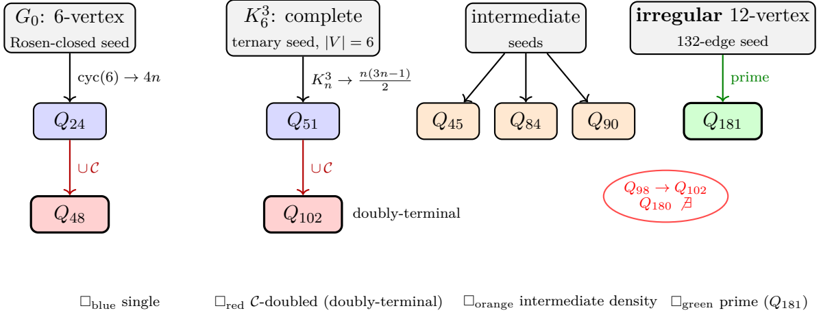
Figure 2: The CFS closure-quotient landscape. Seeds (top row) generate canonical Q_n values (middle); \mathcal{C} -doubling produces the doubly-terminal Q_{48}, Q_{102} (bottom). Two prior-literature entries are corrected in this paper: the previously-reported Q_{98} is a Float64 fidelity-clustering artefact for Q_{102} (§4, [8]); the claimed Q_{180} does not exist because \mathcal{C} is idempotent on \mathcal{C} -closed objects (§4). Q_{181} is the only known prime closure object: it arises from an irregular 12-vertex / 132-edge seed that does not factor through a \text{cyc}(n) or K_n^3 family. Both \text{cyc}(n) \rightarrow 4n and the pentagonal law K_n^3 \rightarrow n(3n-1)/2 are validated exactly on the tested ranges (§5).
