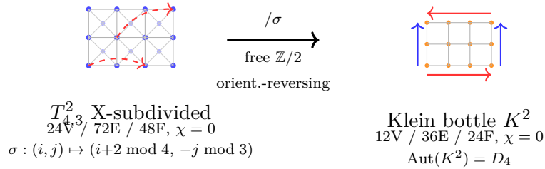
Figure 11: Klein bottle K^2 as the free \mathbb{Z}/2 quotient of the X-subdivided torus T_{4,3}^2 by the orientation-reversing involution \sigma: (i, j) \mapsto ((i+2) \bmod 4, (-j) \bmod 3) . Solid blue dots are corner vertices (12); pale dots are cell-centre vertices (12). Two illustrative \sigma -orbits are shown as red dashed arcs on the left. The quotient K^2 inherits its automorphism structure from the centralizer of \sigma in \text{Aut}(T_{4,3}^2\text{-X-subdiv}) : the \mathbb{Z}_3 translations \tau_{(0,b)} do not commute with \sigma (since -b \neq b in \mathbb{Z}_3 for b \neq 0 ), leaving Z(\sigma) = \mathbb{Z}_4 \rtimes (\mathbb{Z}_2 \times \mathbb{Z}_2) of order 16; modulo \langle \sigma \rangle , the relation \tau_x^2 \equiv \rho_j absorbs \rho_j , yielding \text{Aut}(K^2) = D_4 of order 8. The horizontal double-arrow on K^2 (blue) indicates periodic identification; the anti-parallel vertical arrows (red) indicate the orientation-reversing identification that distinguishes K^2 from T^2 .
