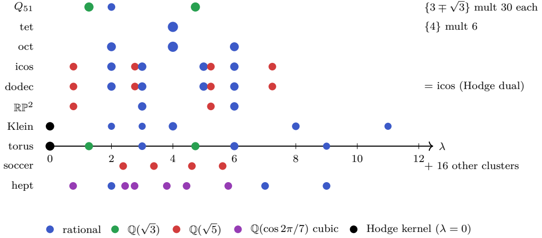
Figure 14: L_1 spectra across the 10-substrate corpus. Each row plots the distinct eigenvalues of L_1(X) on the \lambda -axis as coloured dots; multiplicities are not encoded by dot size (see Table 10 for full multiplicities). Colour encodes Galois content: rational eigenvalues in blue; \mathbb{Q}(\sqrt{3}) Galois pairs in green; \mathbb{Q}(\sqrt{5}) pairs in red; cubic \mathbb{Q}(\cos 2\pi/7) orbits in purple. Black dots at \lambda = 0 mark the Hodge kernel on the Klein bottle (kernel dim 1) and torus (kernel dim 2). The same \mathbb{Q}(\sqrt{3}) pair \{3 \pm \sqrt{3}\} appears in both Q_{51} and the torus T_{3,3}^2 . All four A_5 substrates (icos, dodec, \mathbb{RP}^2 , soccer) carry \mathbb{Q}(\sqrt{5}) pairs with substrate-dependent rational coefficients (icos: \{3 \pm \sqrt{5}, 5 \pm \sqrt{5}\} ; soccer: \{(7 \pm \sqrt{5})/2, (9 \pm \sqrt{5})/2\} ). The heptagonal bipyramid exhibits the only cubic orbits.
