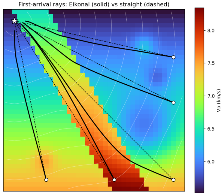
Figure 4: Why the forward operator matters. Solid: Eikonal first-arrival rays, bending through the medium. Dashed: the straight-ray approximation.
