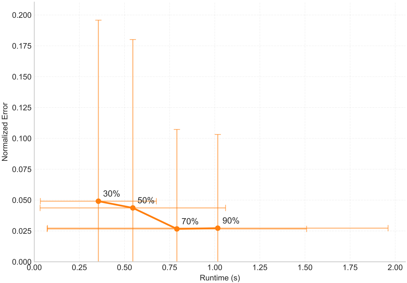
Magic: normalized error vs runtime
