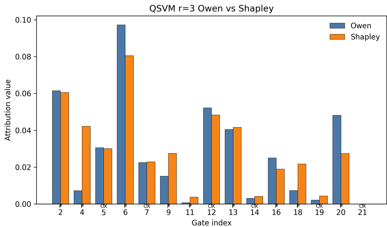
Fig. 13. Gate-level comparison between QSVM Owen values and locked-passive Shapley values for r = 3 . Hadamard gates are passive in both calculations.
