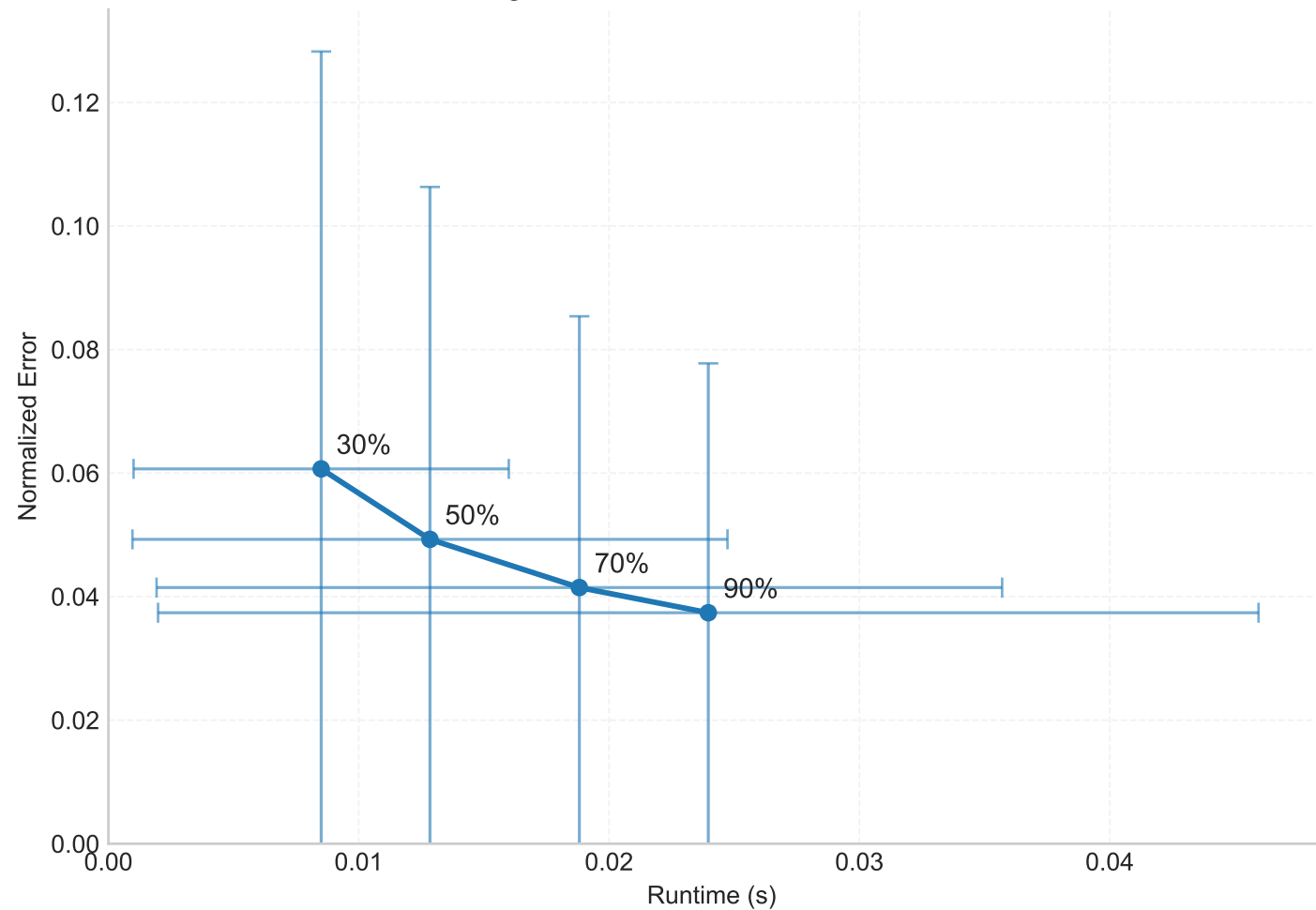
Entanglement: normalized error vs runtime
