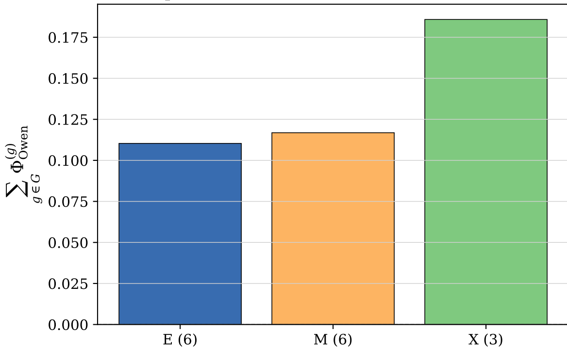
Group-level exact Owen values for QSVM, r=3
