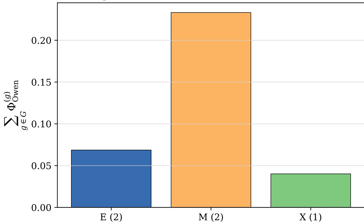
Group-level exact Owen values for QSVM, r=1
