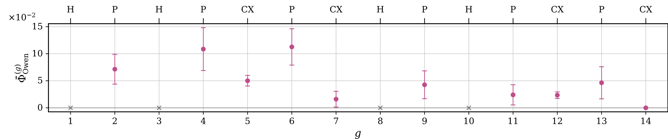
(b) r=2 , exact Owen, mean \pm std over 5 datasets
