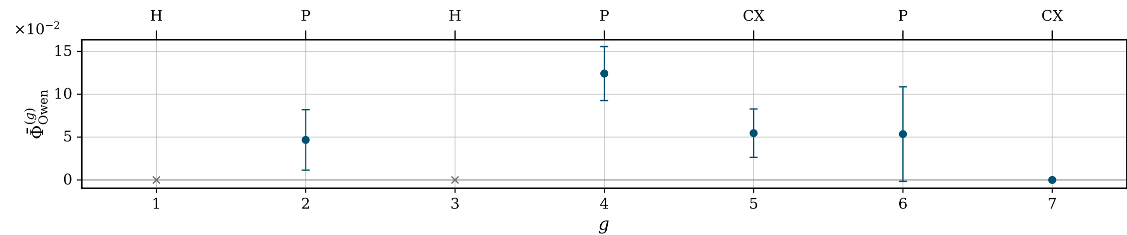
(a) r=1 , exact Owen, mean \pm std over 5 datasets
