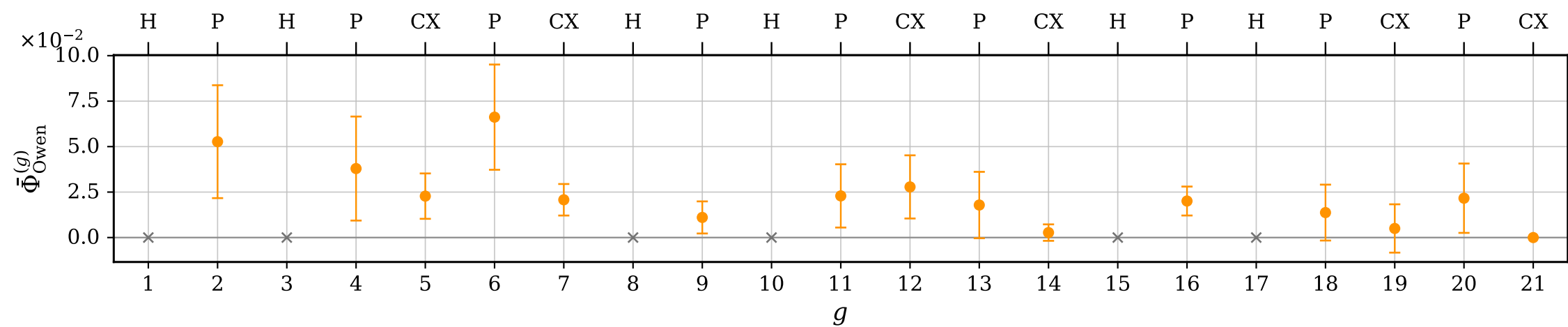
(c) r=3 , exact Owen, mean \pm std over 5 datasets
